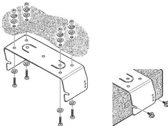
MMB-83 Installation
